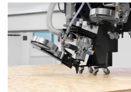
Swiveling units for nailing devices
