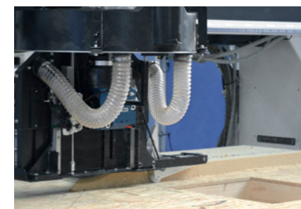
Flex 25 sawing unit
