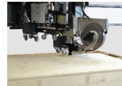
Nail pusher
